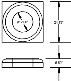
B18 Base for 18" column
