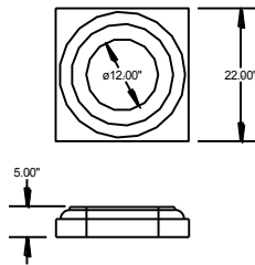
B16C18 Cap for 18" column and base for 16" column
