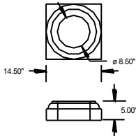
B12C14 Cap for 14" column and base for 12" column
