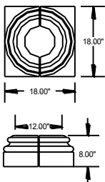
CB - 62408 Base for 12" column
