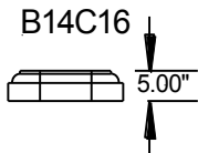
CC - 62008 Cap for 12" column
