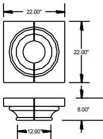
CC - 62008 Cap for 12" column
