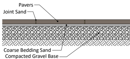
Sand Set
