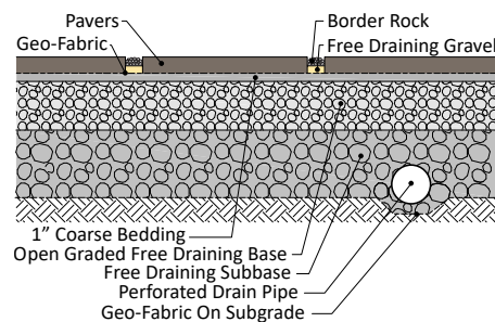
Permeable Set
