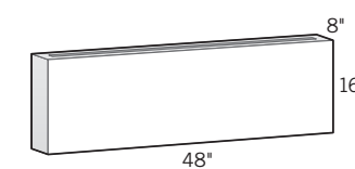
Wilmington Gas-Burning Fireplace Hearth Extension Backrest 8" D × 48" L × 16" H • OLPW81648
