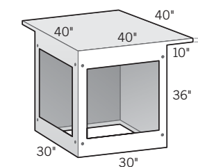
90° Corner Cabinet with 10" Cantilever on Two Sides 30" d × 30" L × 36" h • OLPLSCHBC
