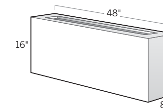
Straight Seating Wall 8" d × 48" L × 16" h • OLPW81648 Create seating walls in hours vs. days. Finish with Eldorado Stone & Wall Caps for an authentic masonry appearance.
