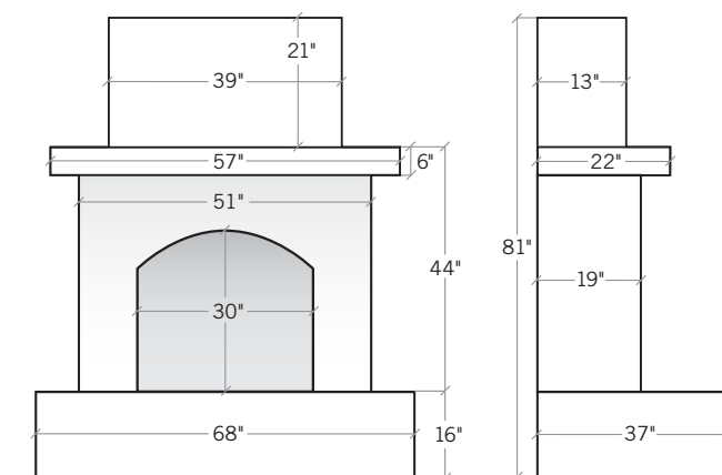
Wilmington Gas-Burning Fireplace 37" D × 68" L × 81" H • OLPLSF01
