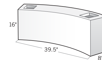
Curved Seating Wall (1/8 Circle) 8" d × 39.5" L × 16" h • OLPW81640 Curved seating wall is designed with a 51" radius from the center point to the inside edge, perfect for pairing with our round fire pit.
