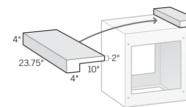
Straight Raised Backsplash OLPLSBSTR Creates 4" high raised backsplash (23.75" long) with 10" cantilever and 14" counter surface. Requires 3 bolts for mounting (not included).
