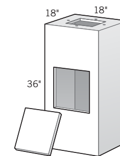
Column with End Cap 18" d × 18" L × 36" h • OLPLS1836 Instantly build perfect stone or brick columns. Column ships with access panel. Designed with top and bottom flange for attaching masonry anchor or bolting.
