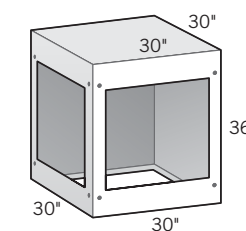
90° Corner Cabinet 30" d × 30" L × 36" h • OLPLS00CN
