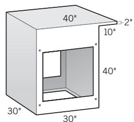
BAR-HEIGHT Cabinet with 10" Cantilever Backside 30" d × 30" L × 40" h • OLPLSBHBS
